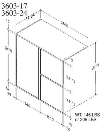
DOUBLE WIDTH, (1) MULTI-TASK LOCKER AND (2) MANAGER/CASH LOCKERS, 32-1/2" W x 30-7/8" H x 17" D or 24" D
